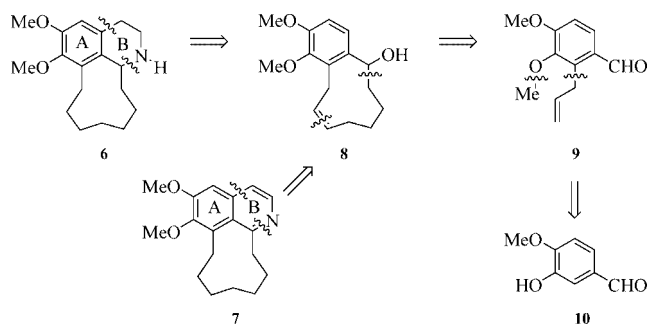
Scheme 1. Retrosynthetic analysis of compounds 6 and 7 .
