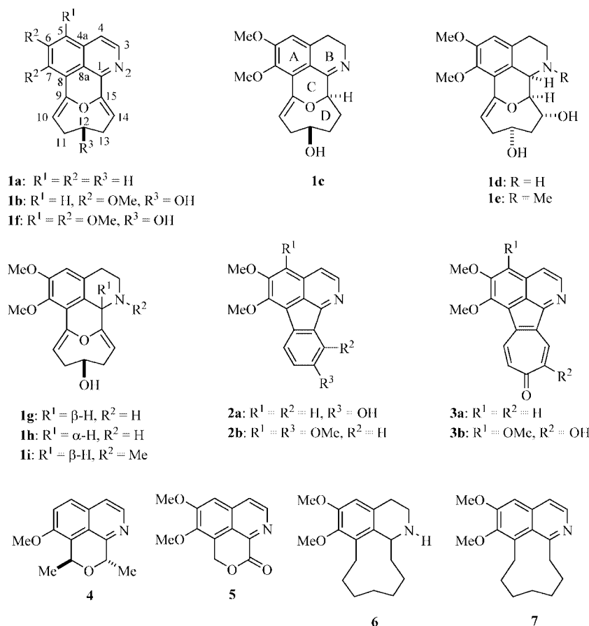
Figure 1. Chemical structures of the stephaxoxanes 1a–i , related natural products 2 and 3 , synthetic tricyclic analogs 4 and 5 and proposed targets 6 and 7 .
