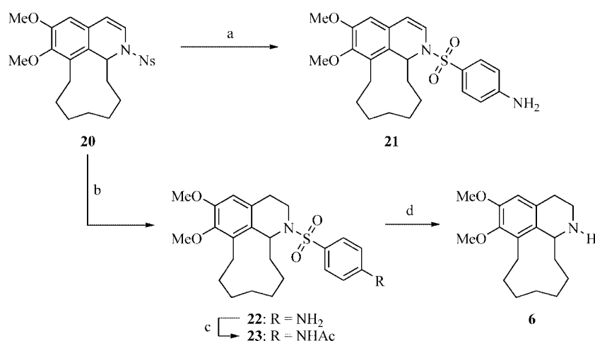
Scheme 3. Nosylamide-based synthesis of compound 6 . Reagents and conditions: a) H 2 (1 atm), 10% Pd/C, MeOH, room temp., 2.5 h (100%); b) H 2 (6 atm), 10% Pd/C, MeOH, room temp., 2.5 h; c) Ac 2 O, pyridine, DMAP (cat.), CH 2 Cl 2 , r.t. (74% overall); d) 1. Na, NH 3 , –33 °C; 2. NH 4 Cl (96%).
