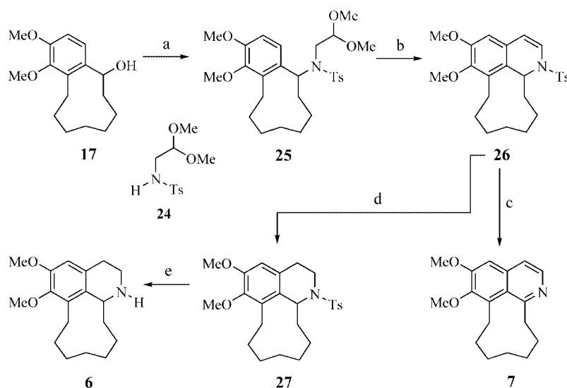
Scheme 4. Tosylamide-based synthesis of compounds 6 and 7 . Reagents and conditions: a) TsNHCH 2 CH(OMe) 2 ( 24 ), PPh 3 , DIAD, THF, room temp., 12 h (68%); b) 6 N HCl, EtOH, dioxane, reflux (50%); c) KtBuO, 2,6-lutidine, 140 °C (70%); d) 1. H 2 (7 atm), 10% Pd/C, MeOH, r.t. 24 h (100%); e) 1. Na, NH 3 , –33 °C; 2. NH 4 Cl (98%).
